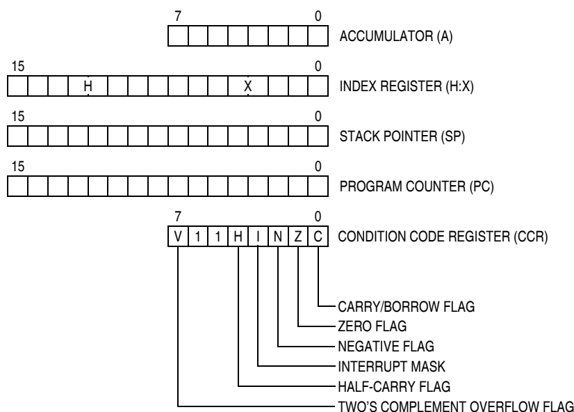
Figure 7-1. CPU Registers
