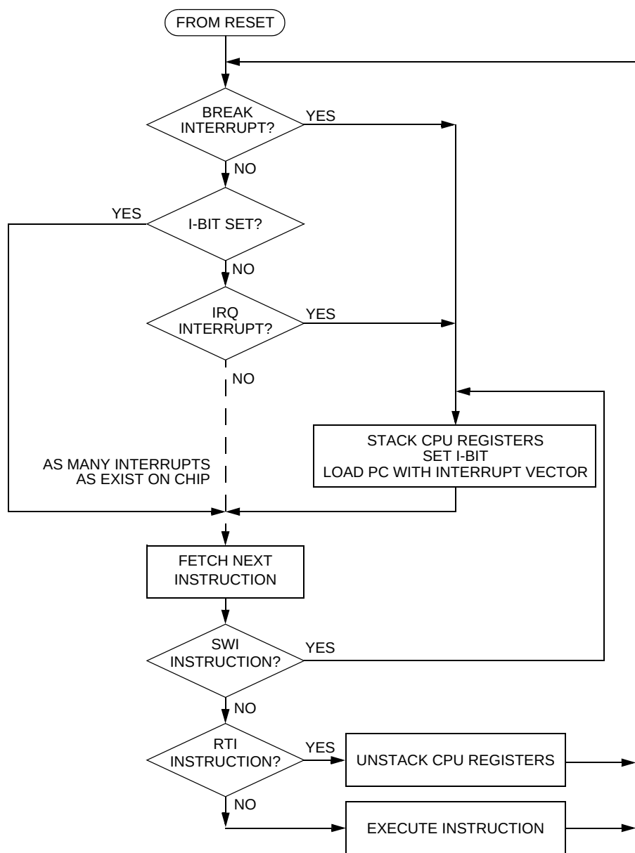
Figure 8-10. Interrupt Processing
