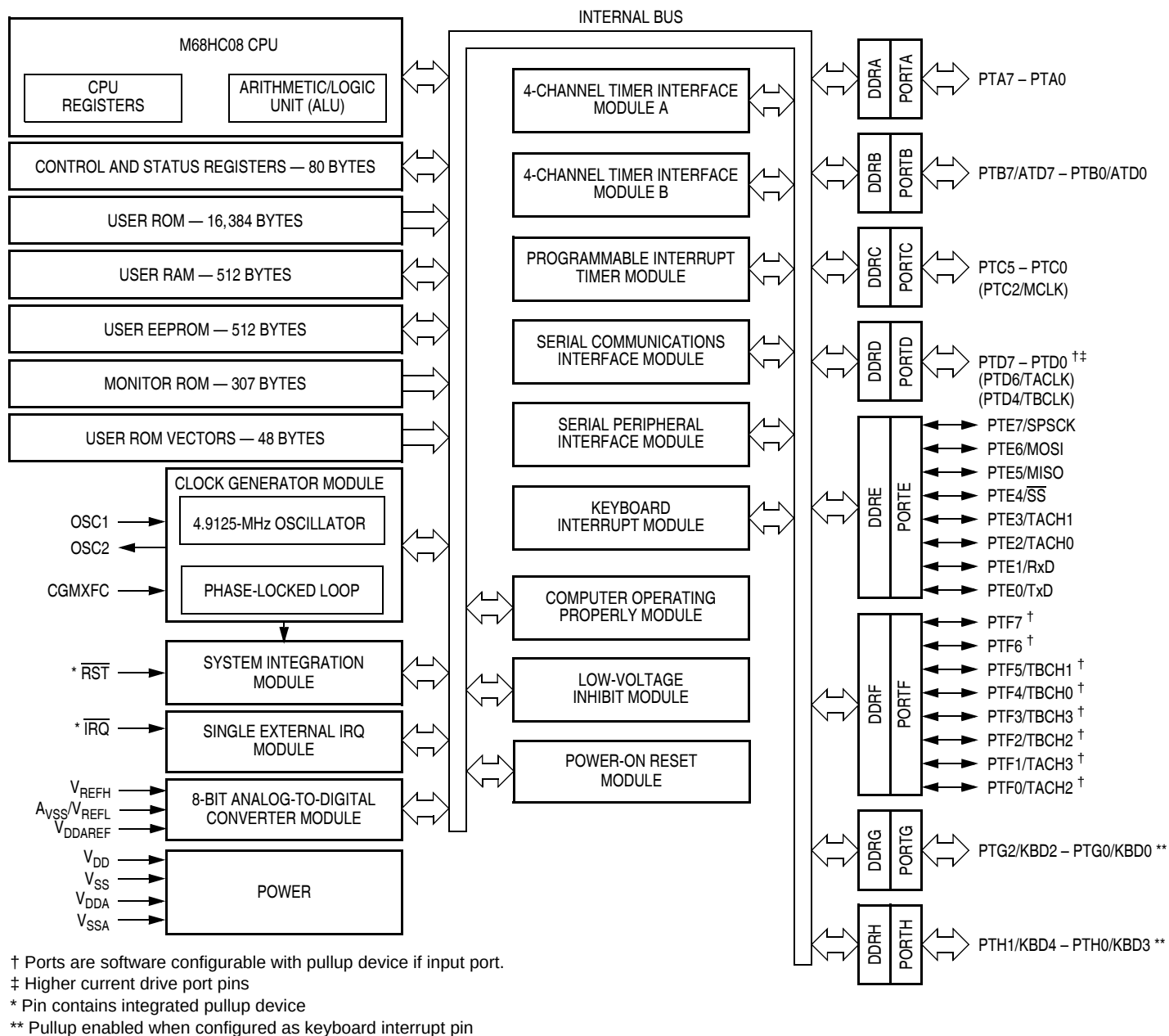
Figure 1-1. MC68HC08AB16A Block Diagram
