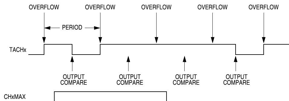
Figure 11-13. CHxMAX Latency
